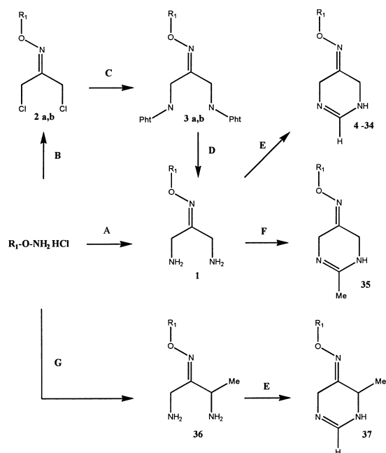
Scheme 1. Synthesis of dihydropyrimidine oxime derivatives. (A) O=C(CH_2NH_2)_2 , MeOH, 20–96 h reflux; (B) O=(CH_2Cl)_2 , MeOH, 2 h, 40 °C; (C) Ph 4 NK, DMF, 4 h, 100 °C; (D) NaONH 2 , MeOH, 2 h, rt; (E) HC(OCH_3)_3 , MeOH, 20 h, reflux; (F) CH_3C(OCH_3)_3 , MeOH, 20 h reflux; (G) H_2NH_2C(C=O)CH(CH_3)NH_2 , MeOH, 20 h reflux.
