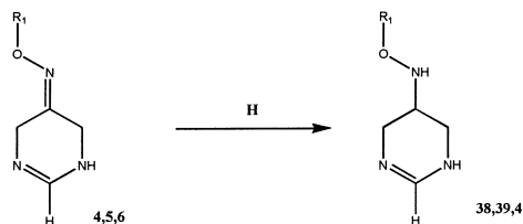
Scheme 2. Synthesis of tetrahydro- N -alkoxy-5-pyrimidinamine derivatives. (H) Trimethylamine–borohydride complex, HCl/MeOH, 2 h, rt.
